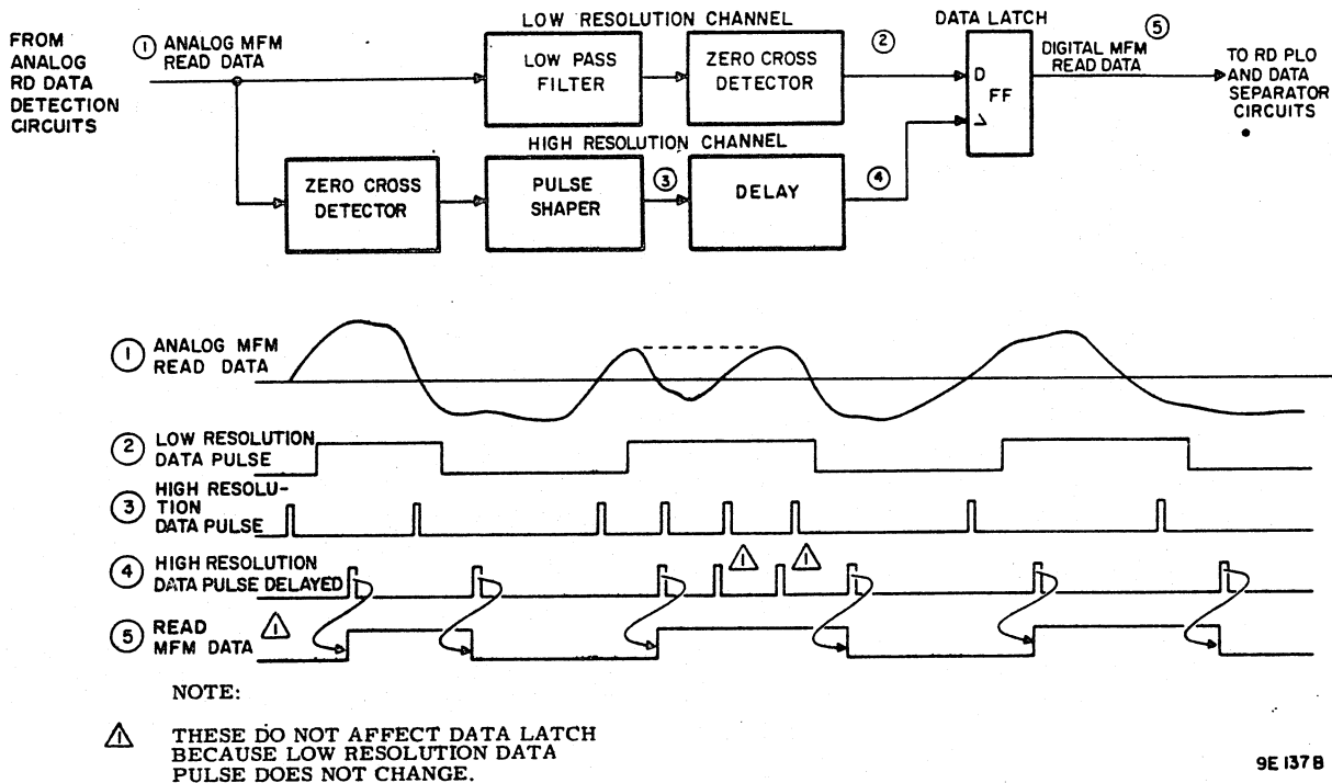
Figure 3-47. Read Analog To Digital Converter Logic and Timing
