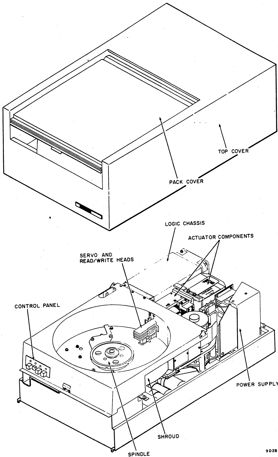
Figure 1-4. Assembly Locations
