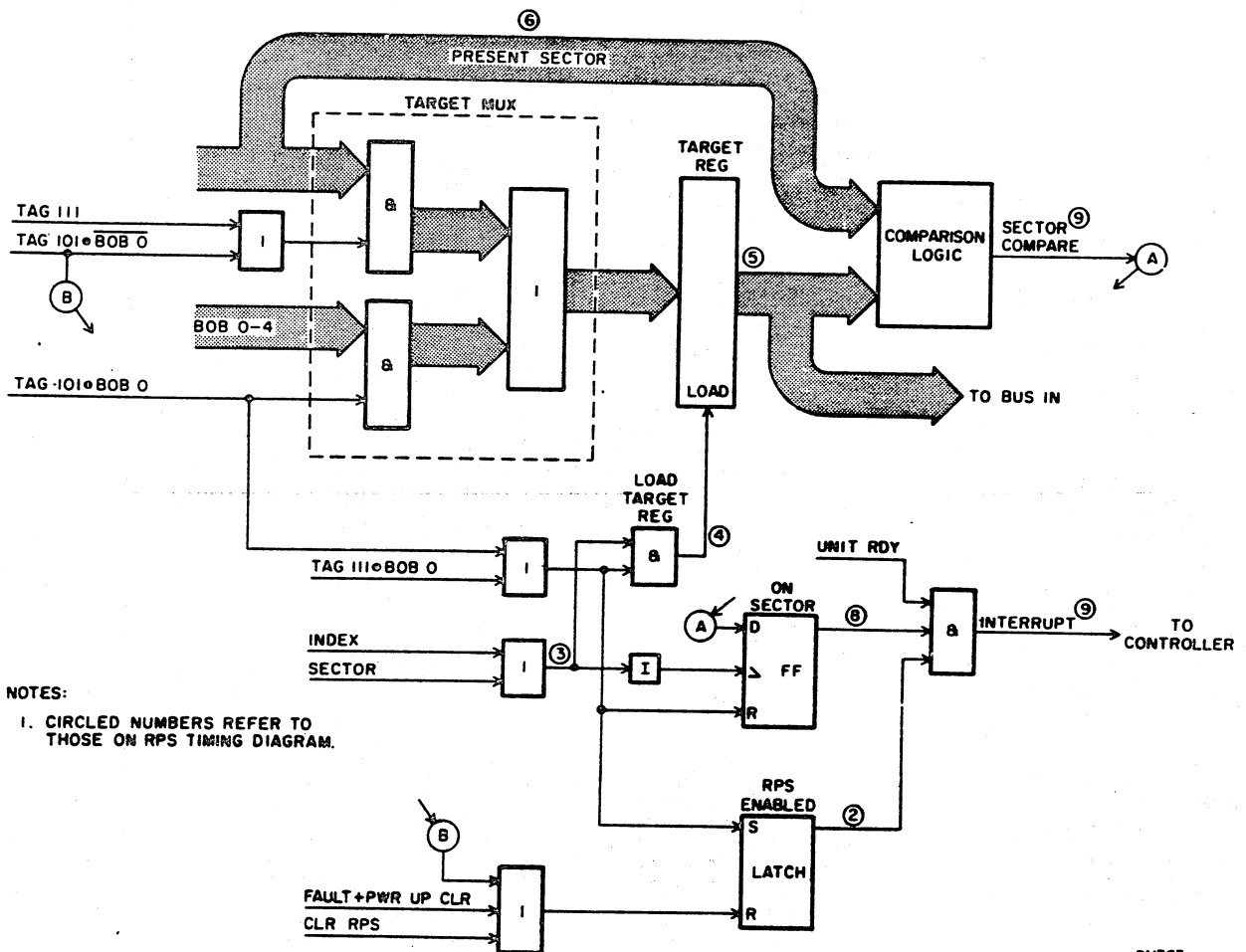
Figure 3-37. RPS Logic
